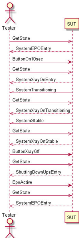
Fig. 9. Generated Sequence Diagram of a Test Case
