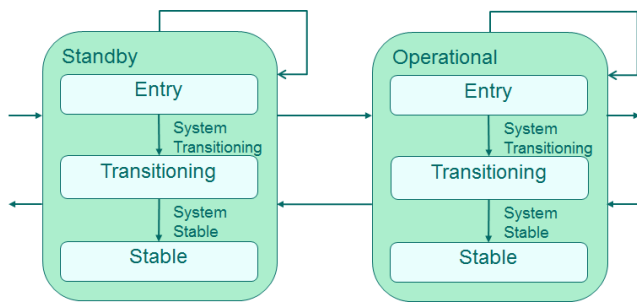
Fig. 3. Two main states and their substates
